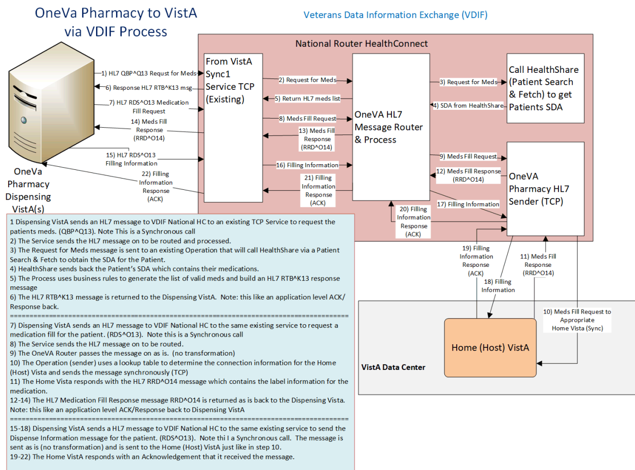
Figure 1: Dispensing VistA Instance to National HL7 Health Connect
