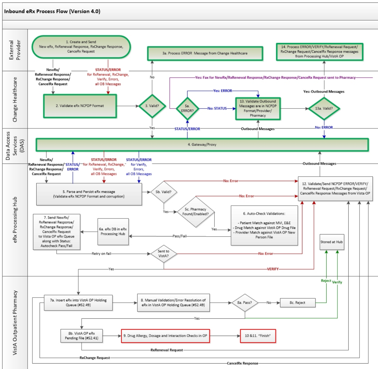
Figure 6: Inbound ePrescribing Process Flow (Version 4.0)
