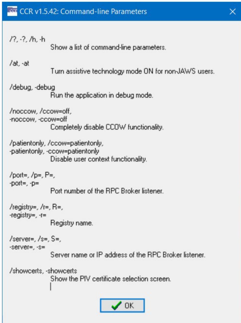
Figure 10 – Command-Line Switches
