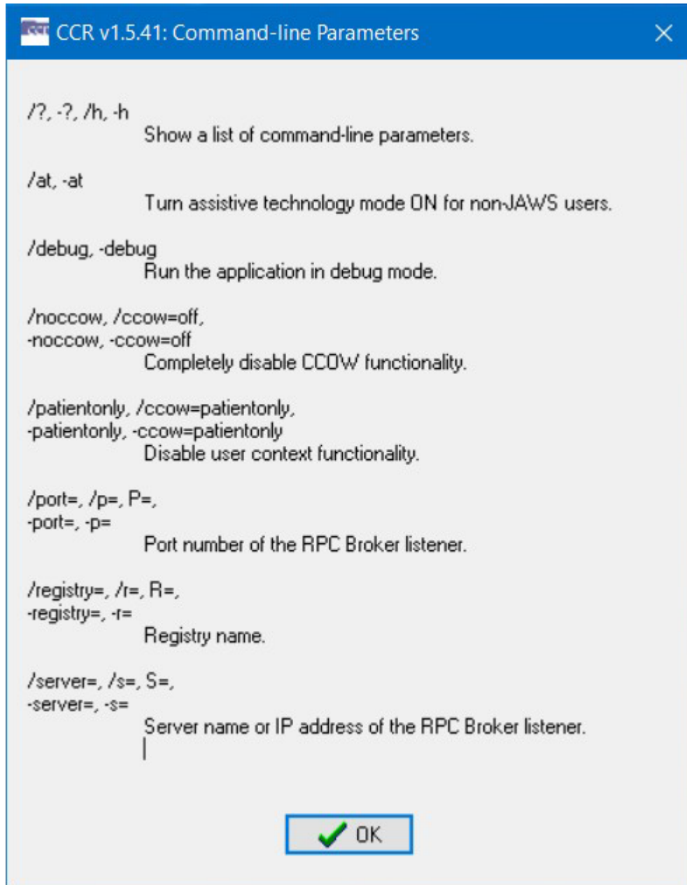
Figure 10 – Command-Line Switches
