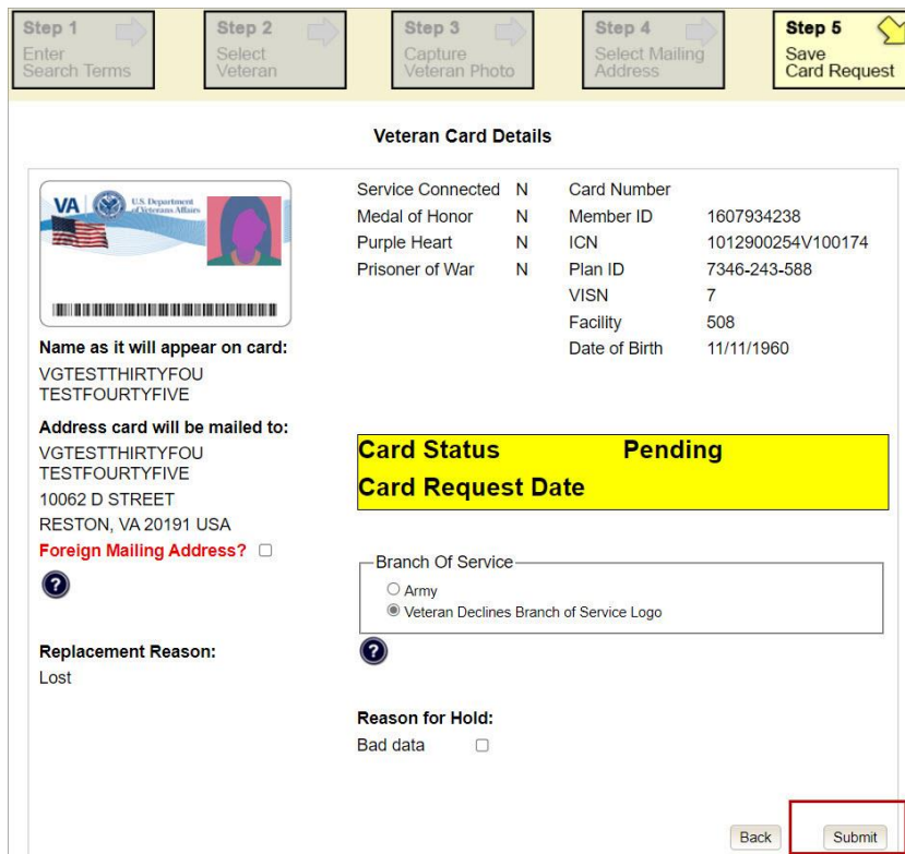
Figure 16: Step 5: Save card Request review screen
