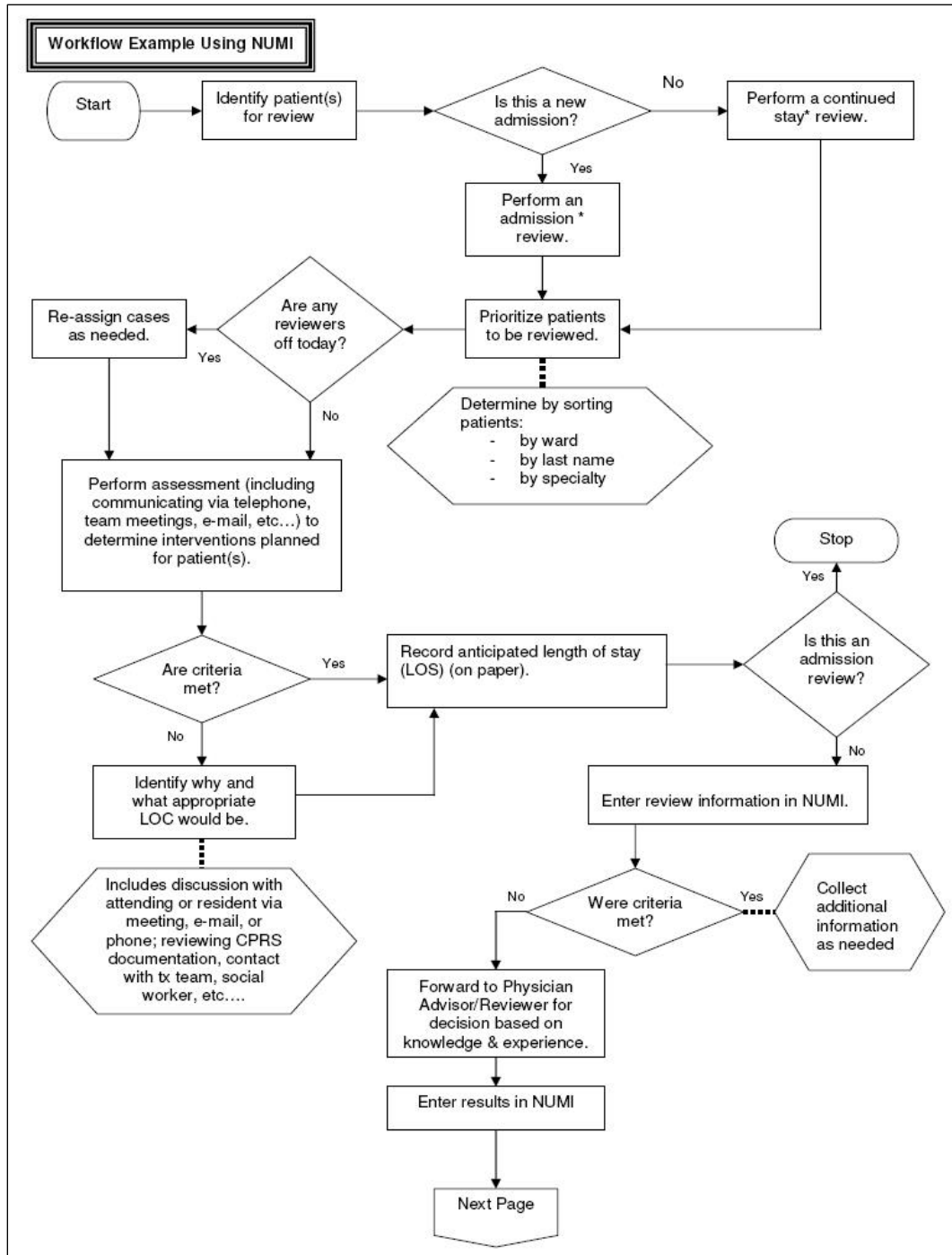
Figure 6: NUMI Workflow Example (part 1)
